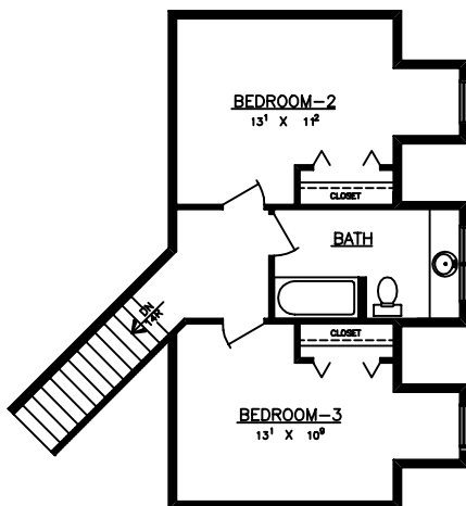
SECOND FLOOR PLAN AREA = 490 S.F.
